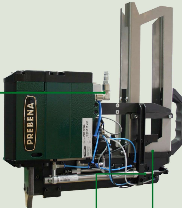
Vertical compressed air connection
